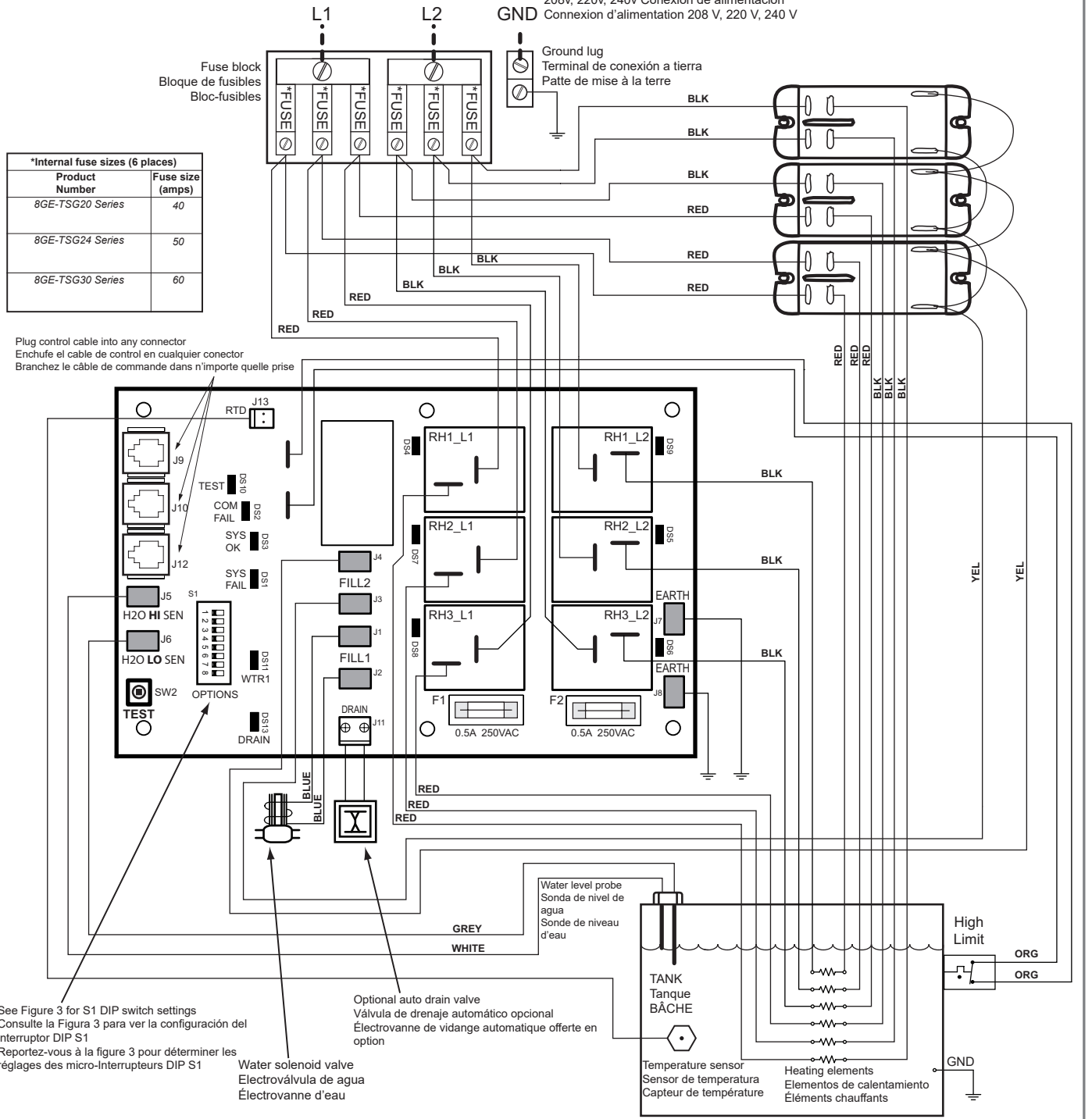
Figure 4 - Wiring Diagram - Single Phase Figura 4 - Diagrama de cableado - Monofásico Figure 4 – Schéma de câblage monophasé
